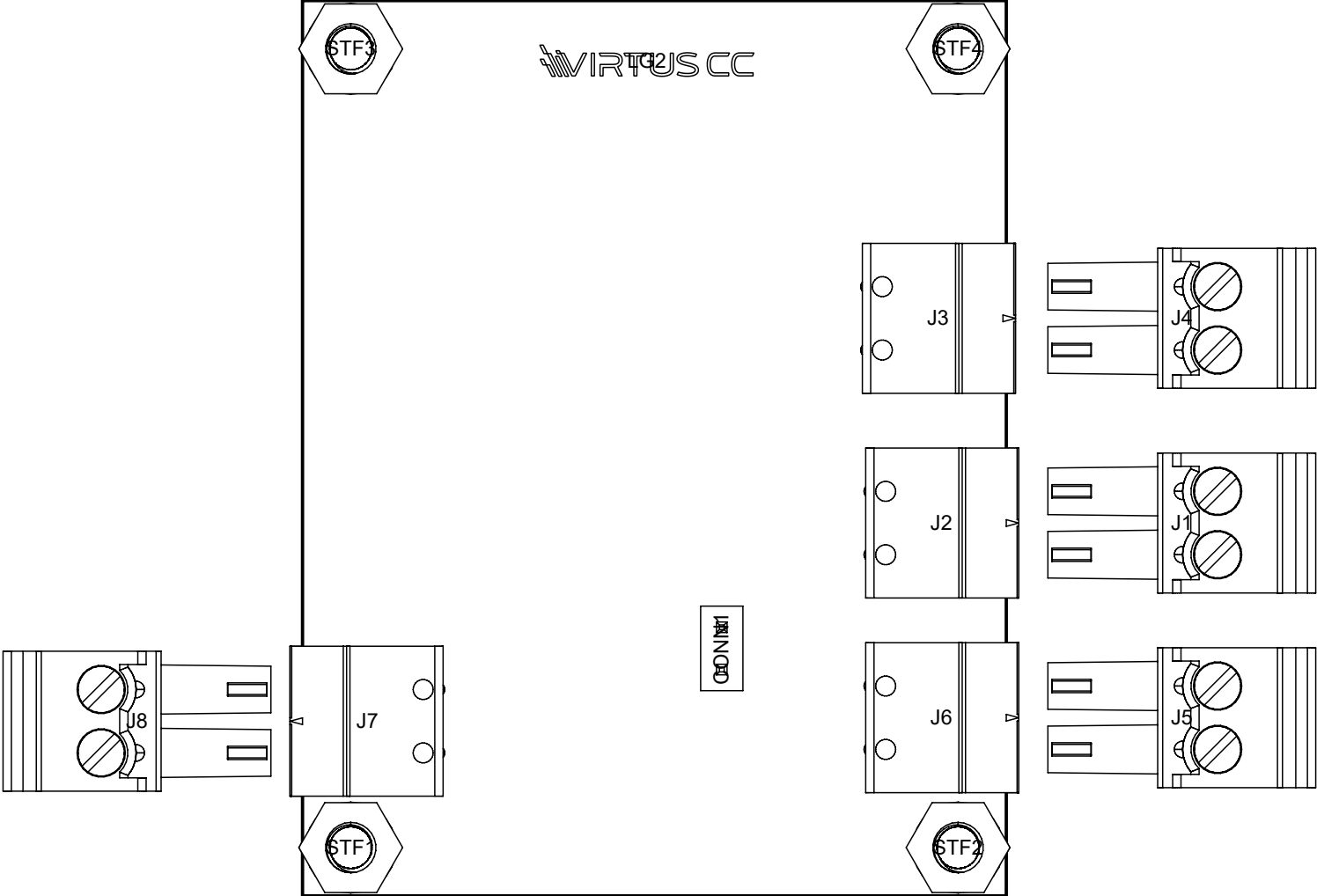
View from Bottom side (Scale 5:2)
